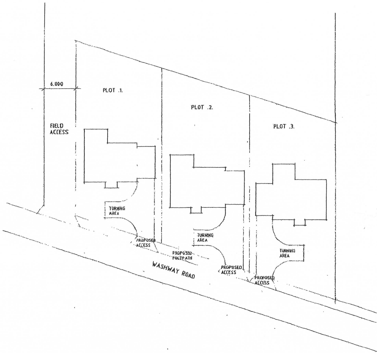
SITE LAYOUT
